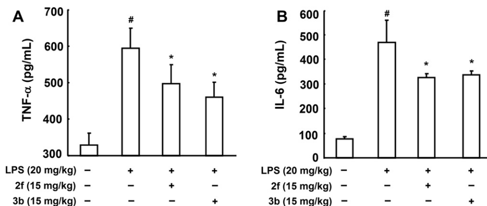
Fig. 4. Effects of 3b and 2f on LPS-induced TNF- \alpha and IL-6 levels in serum ( n = 6 ). Mice were injected (i.p.) with 20 mg/kg LPS. Compounds ( 2f and 3b ) were injected (i.p. 15 mg/kg) once per day for 3 days prior to LPS injection. # p < 0.01 versus blank (without any treatments). * p < 0.05 versus control (treated with LPS only).
