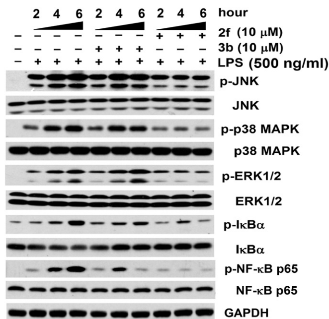
Fig. 1. The effects of compounds 2f and 3b on LPS-induced phosphorylations of JNK, ERK1/2, p38 MAPK, NF-κB p65, and IκBα in RAW264.7 cells. RAW264.7 cells were treated with 2f and 3b (10 μM) and LPS (500 ng/mL). The levels of JNK, ERK1/2, p38 MAPK, NF-κB p65, IκBα, and their phosphorylated forms (p-) at 2, 4 and 6 h incubations in the cellular lysates were analyzed using Western blotting.
