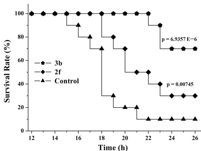
Fig. 3. Effects of 3b and 2f on LPS-induced lethality in mice ( n = 10 ). Mice were injected (i.p.) with 20 mg/kg LPS. Compounds ( 2f or 3b ) were injected (i.p. 15 mg/kg) once per day for 3 days prior to LPS injection. Results were evaluated by the Kaplan–Meier method. The differences between the control group (LPS only) and the treatment groups are statistically significant.
