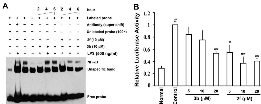
Fig. 2. Effects of 2f and 3b on NF-κB binding to nuclear protein–DNA. (A) Specificity of DNA–protein complex was confirmed with EMSA assay by competition with a 100× excess of unlabeled and p65 of NF-κB antibody supershift assay. (B) RAW264.7 cells transfected with the NF-κB-dependent reporter construct were incubated with LPS (500 ng/mL) in the presence of increasing concentrations of 2f and 3b (5, 10, or 20 μM), then the luciferase activity was measured. Values are means ± SD ( n = 3 ). # p < 0.01 versus normal (without any treatments). * p < 0.05 , ** p < 0.01 versus control (treated with LPS only).
