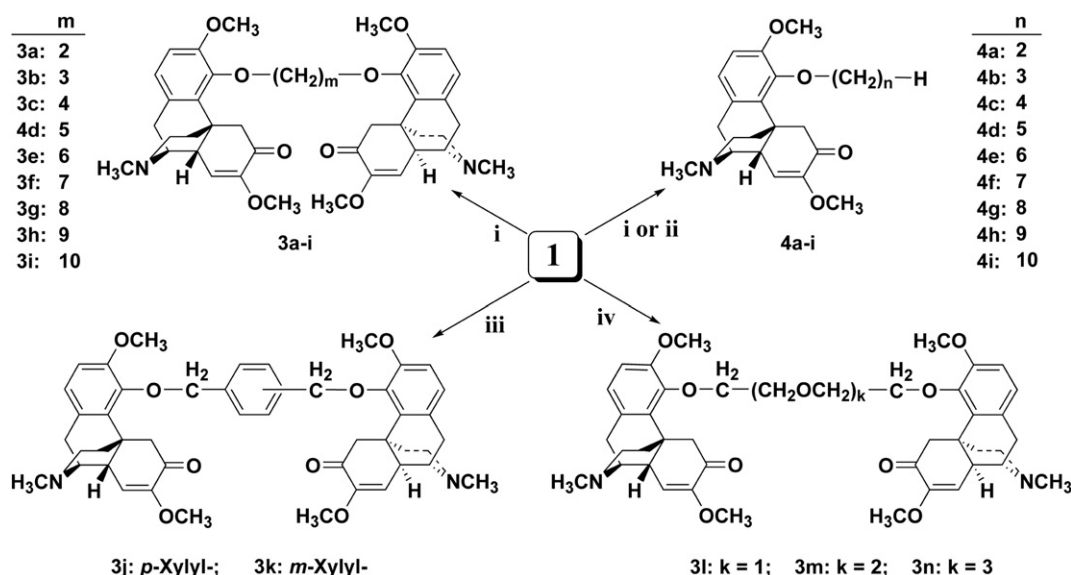
Scheme 2. Synthesis of ether dimers and monomers. Reagents and conditions: (i) Dibromoalkane or bromoalkane, acetone, \text{K}_2\text{CO}_3 , reflux. (ii) Alcohol, DIAD, \text{Ph}_3\text{P} , THF, room temperature. (iii) Xylylene glycol, DIAD, \text{Ph}_3\text{P} , THF, room temperature. (iv) Glycol di- p -tosylate, THF/HMPA (5:1, v/v), NaOH, reflux.
