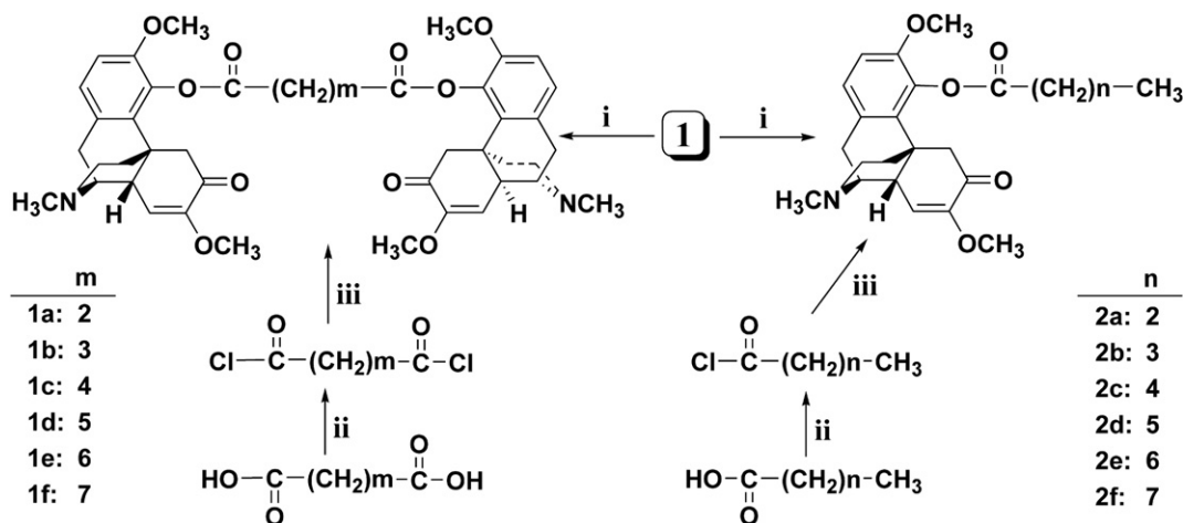
Scheme 1. Synthesis of ester dimers and monomers. Reagents and conditions: (i) DCC, DMAP, CH 2 Cl 2 , room temperature, for 1a , 1c , and 2b–f . (ii) SOCl 2 /DMF (cat.), CH 2 Cl 2 , reflux. (iii) Et 3 N, CH 2 Cl 2 , room temperature, for 1b , 1d–f , and 2a .
