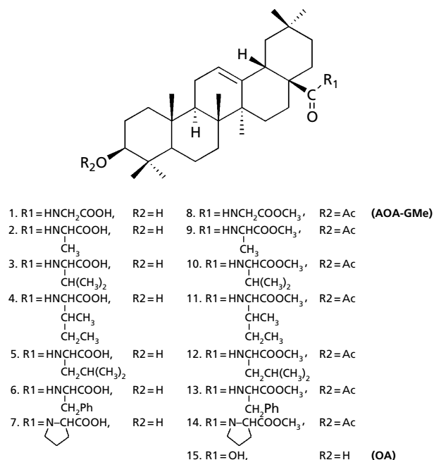
Figure 1 Chemical structures of OA and its derivatives.
